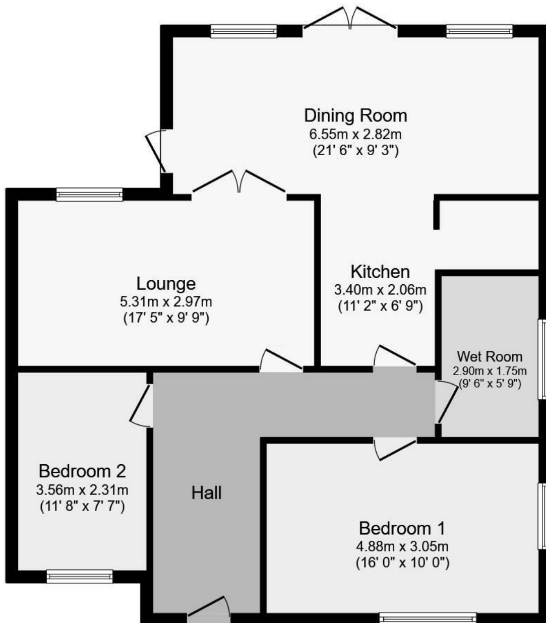
Floor Plan Floor area 86.2 m 2 (927 sq.ft.)
